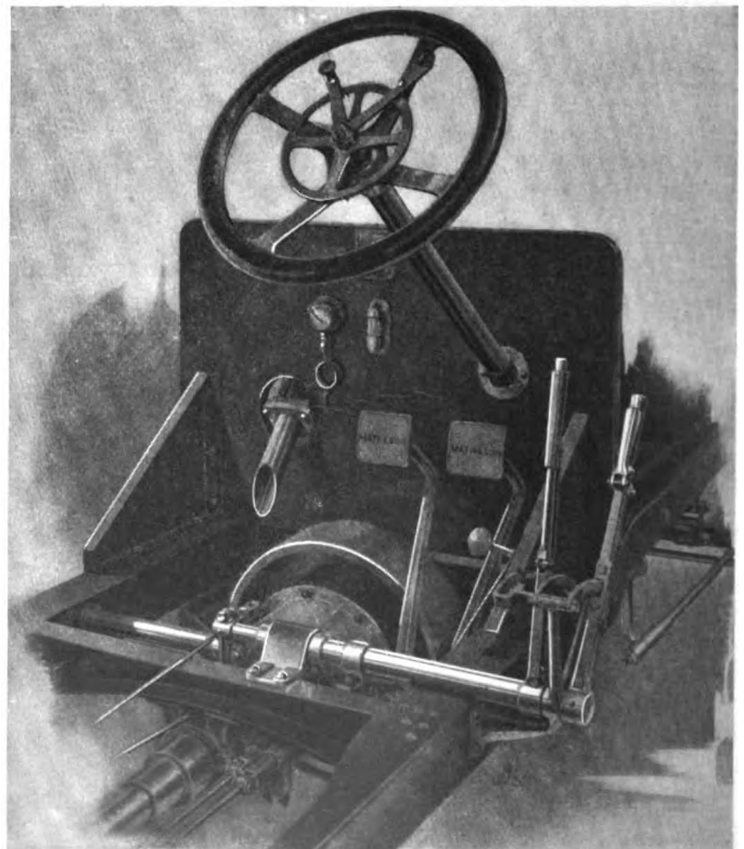
Control Mechanism and Unobstructed Dash.
